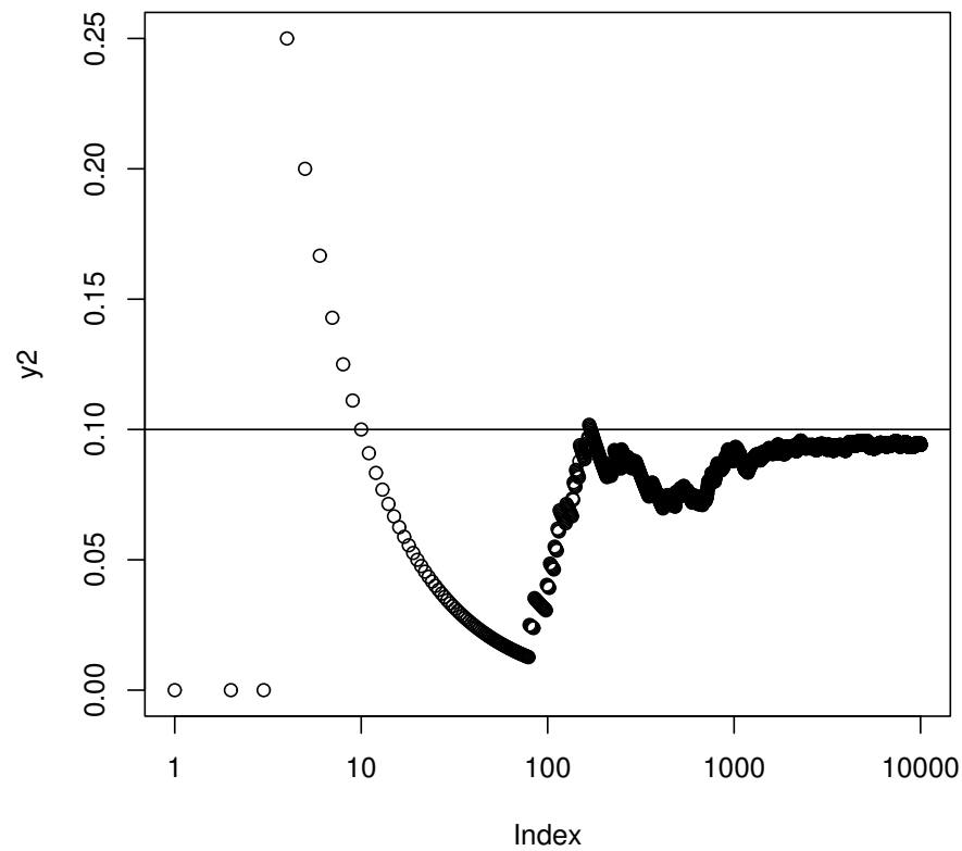
图 6 (左) \bar{Y}_n = \frac{1}{n} \sum_{i=1}^n X_i , (右) \bar{Y}_n = \frac{1}{n} \sum_{i=1}^n I(X_i < 0.1)
