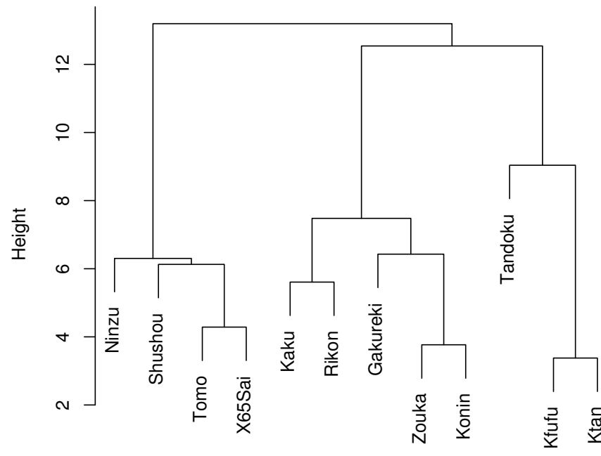
Cluster Dendrogram
